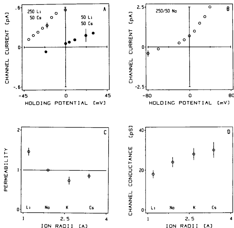
FIGURE 3. Permeability and conductance sequences for alkali cations. A and B correspond to current-voltage curves of single channels in two salts (LiCl-internal, CsCl-external) or single salt (NaCl), respectively. In A data are shown for two separate gradients corresponding to 250 mM Li/50 mM Cs (data points in the upper left quadrant of the I-V curve with a reversal more negative than -40 mV, open circles ) and 50 mM Li/50 mM Cs (data points in the upper right quadrant of the I-V curve with a reversal more negative than 0 mV, filled circles ). In B the ionic condition was 250 mM Na internal/50 mM Na external. Bars (2 SD) are given for data with largest error. C and D correspond to ratios of permeability coefficients and single channel slope conductances (taken at HP 0 mV), respectively. Permeability ratios in C were calculated from Eq. 1 of text and normalized by assuming P(\text{Na}) = 1.0 . Bars, SD of four separate experiments, two determinations in 250 X/50 Y and two determinations in 50 X/50 Y (X, Y test salts) as described in ( A ) and text. The extrapolated zero current potential and the closest data point in the I-V curve were never separated by more than 10 mV. Slope conductance at HP 0 mV in ( D ) were determined for each cation separately in 250 mM internal/50 mM external test cation.
